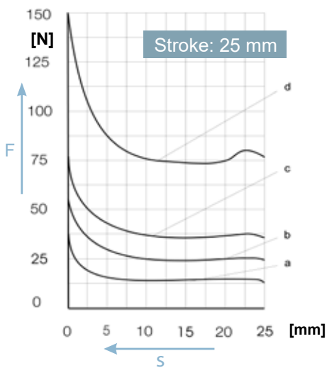
LCL060070 (43 11...06D00/D50)
