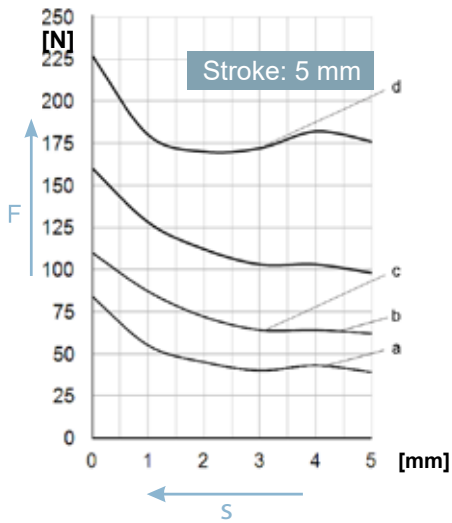
LCL048060 (43 11...05D00/D50)
