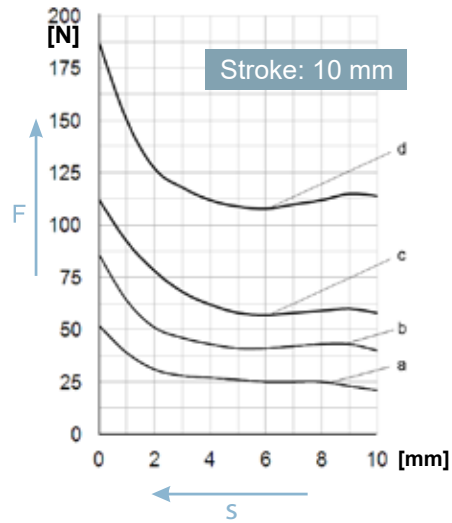
LCL060070 (43 11...06D00/D50)
