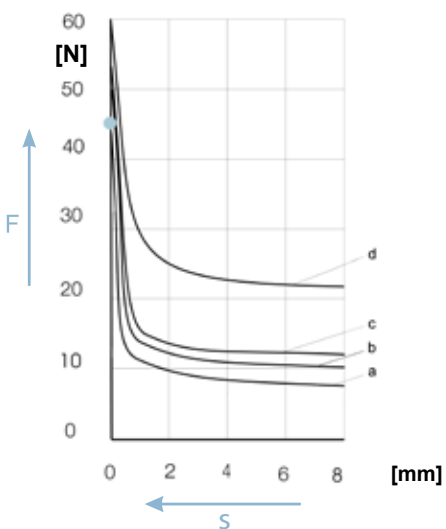
LCM025030A00 (SLP 6030)
