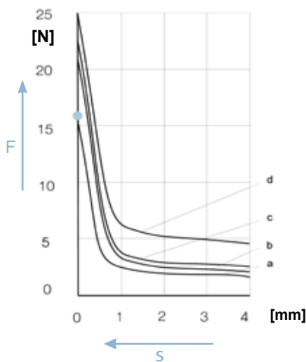
LCM015020A00 (SLP 3020)
