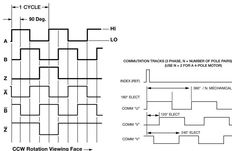
Figure 1 Output Waveform
