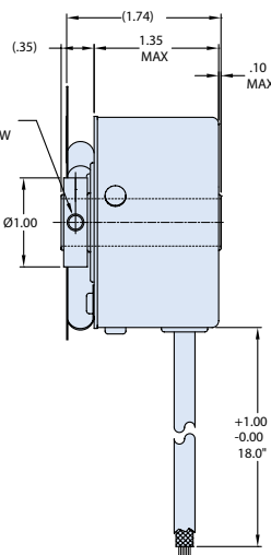
Thru Shaft
