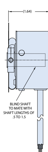
Blind Shaft
