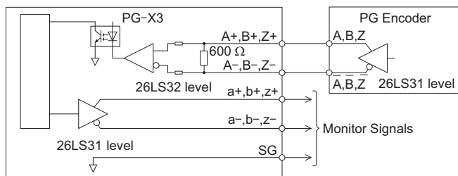
Figure 22 Interface Circuit
