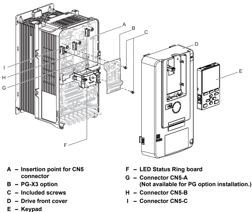
Figure 12 Drive Components with Option
