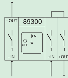
Switching programme 89300
