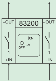
Switching programme 83200
