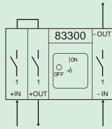
Switching programme 83300
